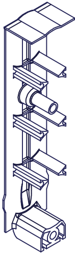
909040 CENTURION QUAD SUPPORT
