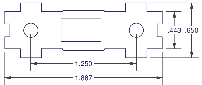
TAB HOUSING
