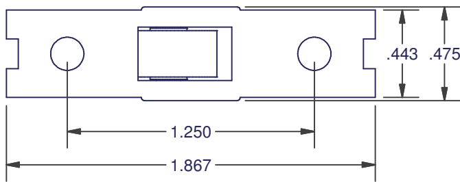
STD HOUSING
